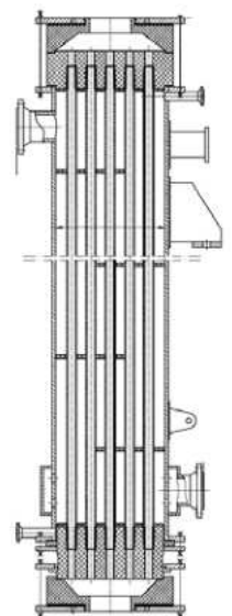
Floating Head
